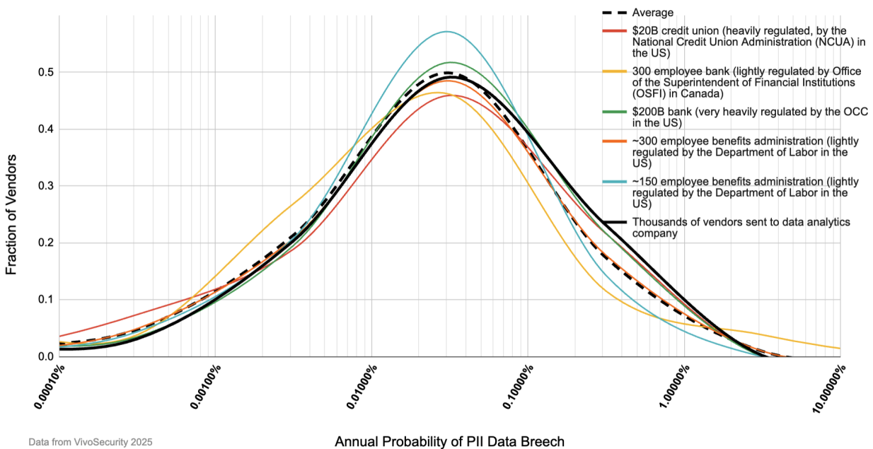
Figure 5, Third-party data breach probability distributions for six organizations chosen to represent a large range in industries, countries, company sizes, numbers of third parties and diverse regulatory regimes.
